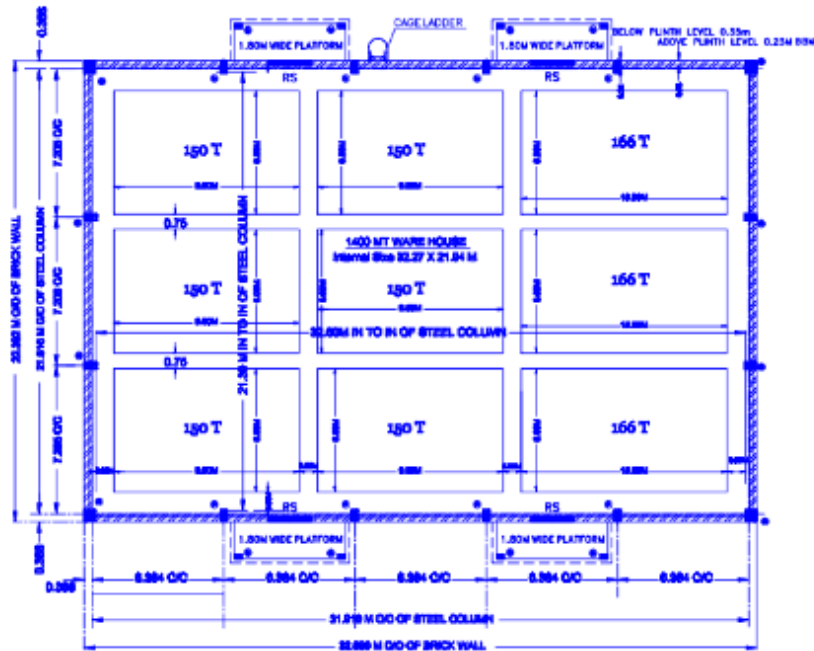
PLAN FOR 1400 MT WARE HOUSE UNIT
